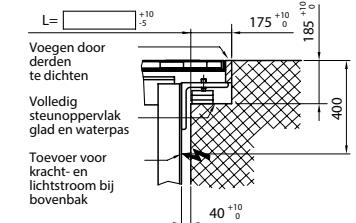
Detail Z
